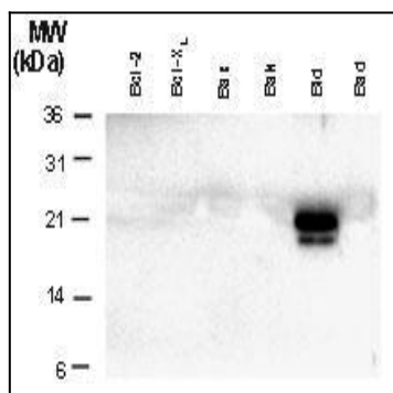
Fig:1 Western blot analysis of Bid using 20-1035 at 1:2000. Detected in vitro translated Bid, but not in vitro translated Bcl-2, Bcl-XL, Bax, or Bad. These results show that 20-1035 is specific for Bid and does not crossreact with other Bcl-2 family members
