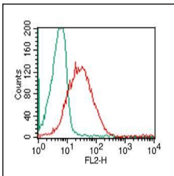
Fig-2: Intracellular flow analysis of HMGB1 in PBMC (Lymphocytes) using 0.5 \mu\text{g}/10^6 cells of HMGB1 antibody (Clone: ABM24C2). Green represents isotype control; red represents anti-HMGB1 antibody. Goat anti-mouse PE conjugate was used as secondary.
