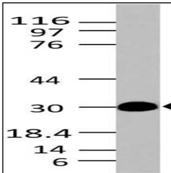
Fig-1: Western blot analysis of HMGB1. Anti- HMGB1 antibody (Clone: ABM24C2) was used at 2 \mu\text{g/ml} on HepG2 lysate.
