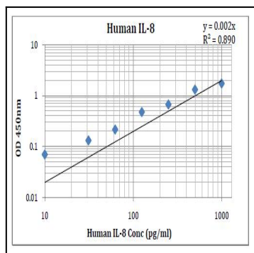
Fig-1:Human IL-8 Standard Curve
