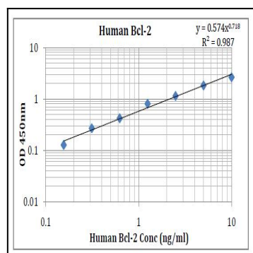
Fig-1: Human Bcl-2 Standard Curve
