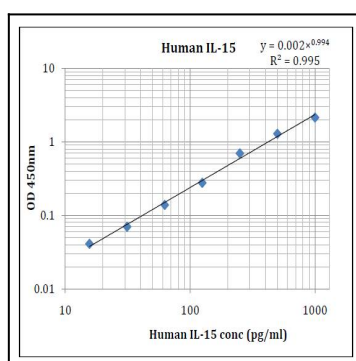
Fig-1: Human IL-15 Standard Curve
