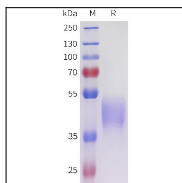
Figure 1. Human ACVR2A(38-106) Protein, mFc Tag on SDS-PAGE under reducing condition.
