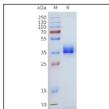
Figure 1. Human PD-L1 Protein, Tag Free on SDS-PAGE under reducing condition.
