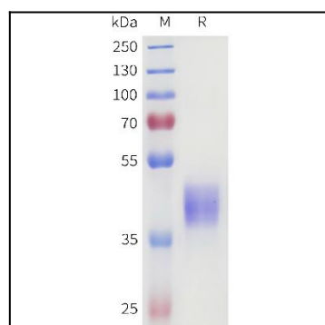
Figure 1. Human 4-1BB(119-160) Protein, hFc Tag on SDS-PAGE under reducing condition.
