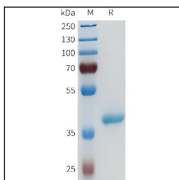
Figure 1. Human ENPP3(94-159) Protein, hFc Tag on SDS-PAGE under reducing condition.
