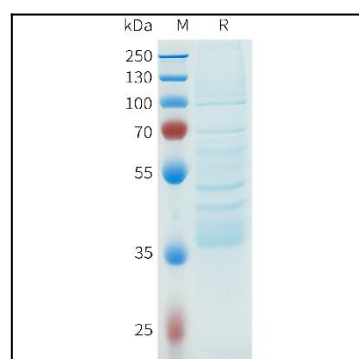
Figure 1. Mouse GDF15 Protein, Flag Tag on SDS-PAGE under reducing condition.
