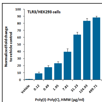
Fig-1: Functional analysis of the TLR3/HEK293 cell line. TLR3/HEK293 cells as well as parental HEK293 cells were transfected with NF-κB/Renilla luciferase reporter plasmid for 16 h. Cells were stimulated with different doses of Poly(I)-Poly(C) (Abeomics, Cat. #15-1012) for 16 h followed by luciferase assay using Luciferase Assay Reagent (Abeomics, Cat. #17-1101).
