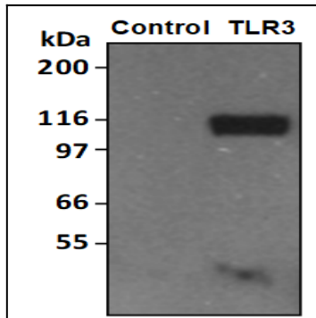
Fig-2: Western blot analysis of TLR3 expression in the TLR3/HEK293 cell line. Cell lysates were analyzed by SDS-PAGE followed by Western blotting using anti-HA antibody. Note that TLR3 in the TLR3/HEK293 stable cell line contains the N-terminal HA tag. Control, parental HEK293 cell lysate; TLR3, TLR3/HEK293 cell lysate.
