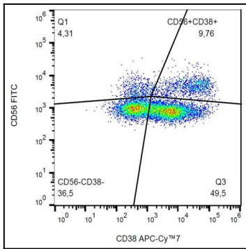
Figure 1: Flow cytometry analysis (surface staining) of human peripheral blood with anti-human CD38 (HIT2) APC-Cy™ 7.
