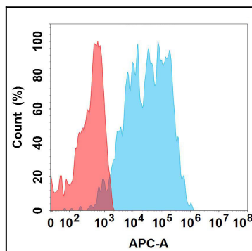
Figure 1. Flow cytometry analysis with 1 \frac{1}{4} g/mL Anti-CD19(loncastuximab biosimilar) mAb on Expi293 cells transfected with Human CD19 protein (Blue histogram) or Expi293 transfected with irrelevant protein (Red histogram).
