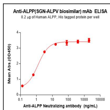
Figure 1. ELISA plate pre-coated by 2 1/4g/mL (100 1/4L/well) Human ALPP Protein, His Tag can bind Anti-ALPP(SGN-ALPV biosimilar) mAb in a linear range of 0.13-3.20 ng/mL.
