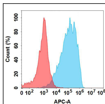
Figure 2. Flow cytometry analysis with 1 1/4g/mL Anti-ALPP(SGN-ALPV biosimilar) mAb on Expi293 cells transfected with Human ALPP protein (Blue histogram) or Expi293 transfected with irrelevant protein (Red histogram).
