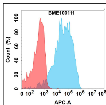
Figure 1. Flow cytometry analysis with 1 \frac{1}{4} g/mL Anti-LRRC15(samrotamab biosimilar) mAb on Expi293 cells transfected with Human LRRC15 protein (Blue histogram) or Expi293 transfected with irrelevant protein (Red histogram).
