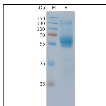
Figure 1. Cynomolgus TIM3 Protein, hFc Tag on SDS-PAGE under reducing condition.
