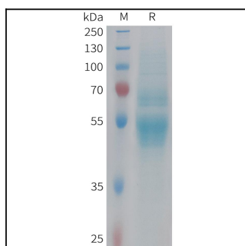
Figure 1. Human F10 Protein, His Tag on SDS-PAGE under reducing condition.
