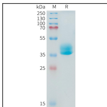
Figure 1. Human ADAM17(581-642) Protein, mFc Tag on SDS-PAGE under reducing condition.
