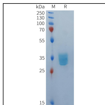
Figure 1. Human BCMA(42-54) Protein, mFc Tag on SDS-PAGE under reducing condition.
