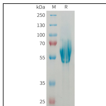
Figure 1. Human MADCAM1 Protein, His Tag on SDS-PAGE under reducing condition.
