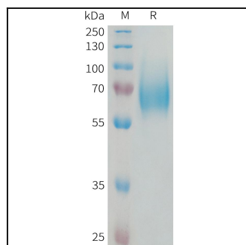
Figure 1. Human FGFR1 Protein, His Tag on SDS-PAGE under reducing condition.
