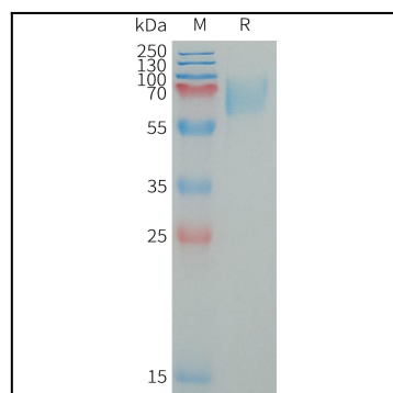
Figure 1. Human LILRA2 Protein, His Tag on SDS-PAGE under reducing condition.
