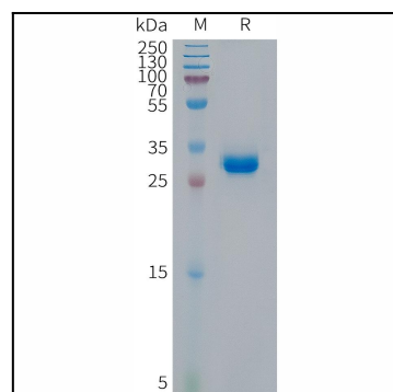
Figure 1. Human p16(11-40) Protein, hFc Tag on SDS-PAGE under reducing condition.
