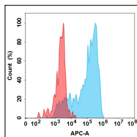
Figure 2. Flow cytometry analysis under cell membrane permeable condition with 1 µg/mL Anti-IL22 (fezakinumab biosimilar) mAb on Expi293 cells transfected with Human IL22 protein (Blue histogram) or Expi293 transfected with irrelevant protein (Red histogram).
