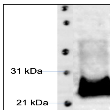
Figure1: Western blot of Monkey pox A35R protein using anti-His antibody.
