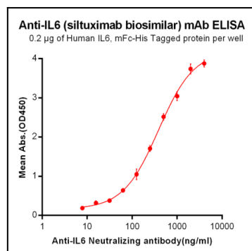
Figure-1: ELISA plate pre-coated by 2 µg/ml (100 µl/well) Human IL6, mFc-His tagged protein can bind Anti-IL6 Neutralizing antibody in a linear range of 7.81-386.8 ng/ml.
