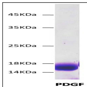
Figure-1: SDS-PAGE analysis of purified Recombinant PDGF Protein was run on a 4-20% Gradient SDS-PAGE (Reducing) gel followed by Coomassie blue staining.
