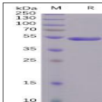
Figure 1. SARS-CoV-2 (2019-nCoV) S1 protein CTD, hFc Tag on SDS-PAGE under reducing condition.
