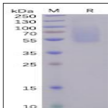
Figure 1. SARS-CoV-2 (2019-nCoV) S1 protein NTD, His Tag on SDS-PAGE under reducing condition.
