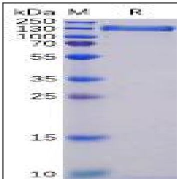
Figure 1. Human ACE2 Protein, hFc Tag on SDS-PAGE under reducing condition.
