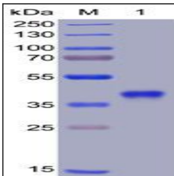
Figure 1. SARS-CoV-2 (2019-nCoV) S protein RBD, His Tag on SDS-PAGE under reducing condition.
