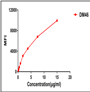
Figure 2. FACS data of serially titrated Rabbit anti-CD138 monoclonal antibody (clone: DM46) on H929 cells. The Y-axis represents the mean fluorescence intensity (MFI) while the X-axis represents the concentration of IgG used.
