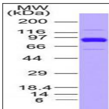
Figure-1: Recombinant SARS-CoV-2 Spike S1 (K417N / E484K / N501Y) mutant protein was run on a 4-20% SDS-PAGE gel followed by Coomassie blue staining.
