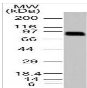
Figure-2: Western blot analysis of SARS-CoV-2 Spike S1 (K417N / E484K / N501Y) mutant protein. Anti-Spike S1 antibody was used in western Blot analysis.
