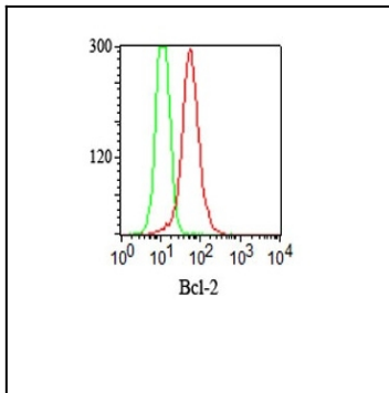
Intracellular staining of Bcl-2 in Jurkat cells using Bcl-2 Monoclonal Antibody (100/D5 + 124) (red) and isotype control (green).
