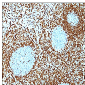
Formalin-fixed, paraffin-embedded human non-Hodgkin's Lymphoma stained with Bcl-2 Monoclonal Antibody (100/D5 + 124). Note nuclear membrane & cytoplasmic staining.
