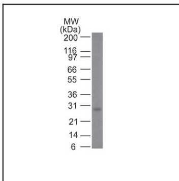
Western Blot of Bcl-2 in human skin using Bcl-2 Monoclonal Antibody (100/D5 + 124).
