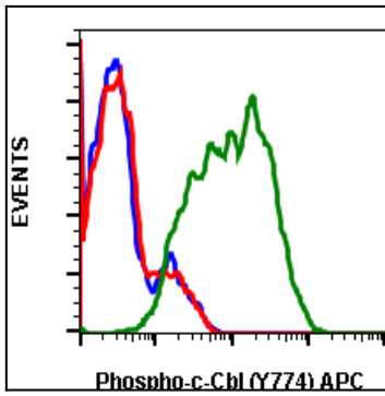
Fig-1: Flow cytometric analysis of Daudi cells cell only (blue) or untreated (red) or treated with IFN \alpha + IL-4 + pervanadate (green) using Phospho-c-Cbl (Tyr774) APC-conjugated antibody CblY774-R3B8.
