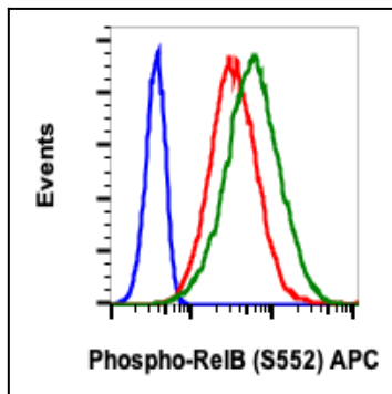
Fig-1: Flow cytometric analysis of NIH3T3 cells untreated and unstained as negative control (blue) or untreated (red) or treated with UV plus TPA (green) and stained using Phospho-ReI B (Ser552) APC-conjugated antibody RelBS552-A7.
