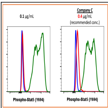
Fig-4: Flow cytometric analysis of 3T3 cells secondary antibody only negative control (blue) or treated with imatinib (red) or with pervanadate (green) using 0.1 µg/mL of Phospho-Stat5 (Tyr694) antibody Stat5Y694-B5 or Company C antibody at 0.4 µg/mL (manufacturer's recommended concentration).
