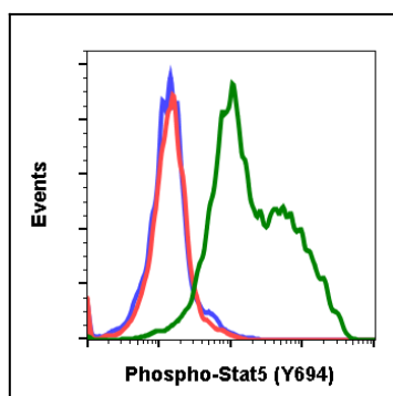
Fig-1: Flow cytometric analysis of K562 cells secondary antibody only negative control (blue) or treated with imatinib (red) or treated with pervanadate (green) using Phospho-Stat5 (Tyr694) antibody Stat5Y694-B5 at 0.05 \mu g/mL.
