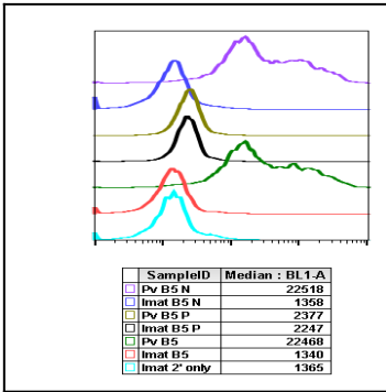
Fig 2 : Peptide blocking flow cytometric analysis of K562 cells secondary antibody only negative control (light blue) or treated with imatinib (red) or pervanadate-treated (green) or imatinib and blocked with phospho-peptide (black) or pervanadate and blocked with phospho peptide (gold) or imatinib and blocked with non-phospho peptide (dark blue) or pervanadate and blocked with non-phospho peptide (purple) using Phospho-Stat5 (Tyr694) antibody Stat5Y694-B5 at 0.1 µg/mL.
