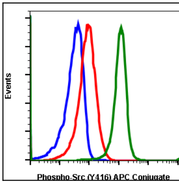
Fig-1: Flow cytometric analysis of U937 cells unstained untreated cells as negative control (blue) or stained and untreated (red) or treated with IFNα IL4 and pervanadate (green) using Phospho-Src (Tyr416) antibody SrcY416-C4 APC conjugate.
