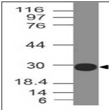
Figure-1: Western Blot analysis of SARS-CoV-2 Spike RBD Antibody: Anti- SARS-CoV-2 Spike RBD Antibody (Clone: ABM5H1.1E4) was used at 0.5 \mu\text{g/ml} on SARS-CoV-2 Spike RBD Recombinant protein.
