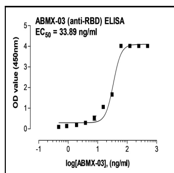
Fig-1: ELISA detection of Anti-SARS-CoV-2 Spike RBD antibody (ABMX-003) cat. no. 10-2006. An ELISA plate coated with 100 ng of full length SARS CoV2 Spike protein (Abeomics, Cat. No. 21-1008) was incubated with various concentrations of Anti-RBD recombinant antibody (ABMX-003). Goat anti-human FC HRP was used as detection antibody.
