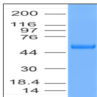
Figure 1: SDS PAGE- Recombinant Sars-Cov-2 Spike RBD Protein Fc Tag (319-541 aa). 5 µg protein was run on a 4-20% SDS-PAGE gel followed by Coomassie blue staining.
