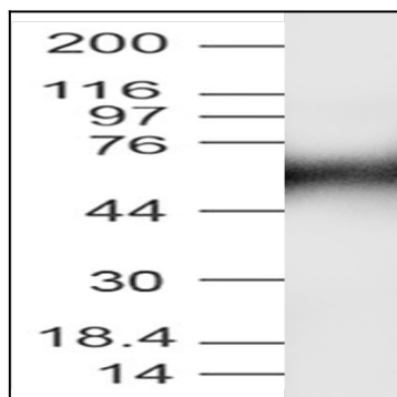
Figure 3: Western Blot analysis of S1-RBD antibody: Anti-S1-RBD antibody (SARS-CoV-2) was used at 2 \mu g/ml on Recombinant Sars-Cov-2 Spike RBD Protein Fc Tag (319-541 aa) (21-1005).
