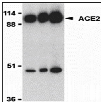
Figure-1: Western blot analysis of ACE2. Anti- ACE2 antibody (35-1877) was used at 0.5, 1, 2 µg/ml on human kidney lysate.
