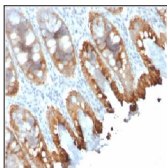
Fig. 1: Formalin-fixed, paraffin-embedded human colon stained with Cytokeratin 8/18 Mouse Recombinant Monoclonal Antibody (rKRT8.18/1346).
