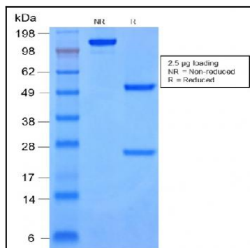
Fig. 2: SDS-PAGE Analysis Purified Cytokeratin 8/18 Mouse Monoclonal Antibody (rKRT8.18/1346).Confirmation of Integrity and Purity of Antibody.
