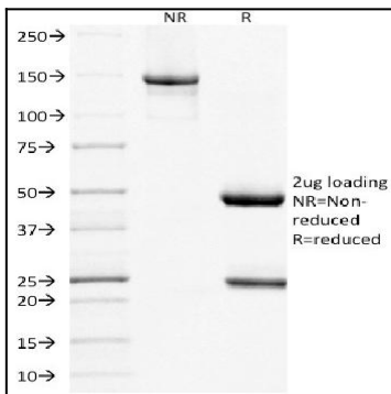
Fig. 2: SDS-PAGE Analysis Purified MUC16 Mouse Monoclonal Antibody (MUC16/1860). Confirmation of Integrity and Purity of Antibody.
