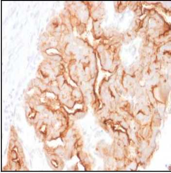
Fig. 1: Formalin-fixed, paraffin-embedded human Ovarian Carcinoma stained with MUC16 Mouse Monoclonal Antibody (MUC16/1860).
