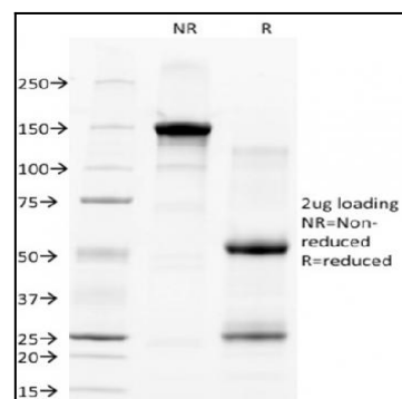
Fig. 1: SDS-PAGE Analysis Purified CD28 Mouse Monoclonal Antibody (C28/77). Confirmation of Integrity and Purity of Antibody.
