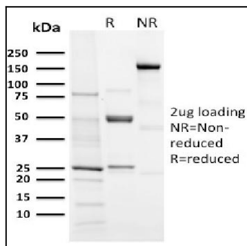
Fig. 2: SDS-PAGE Analysis Purified Aurora B Rabbit Recombinant Monoclonal (AURKB/3121R). Confirmation of Purity and Integrity of Antibody.
