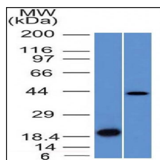
Fig. 1: Western Blot Analysis (A) Recombinant Protein (B) Human Liver lysate Aurora B Mouse Monoclonal Antibody (AURKB/1521).
