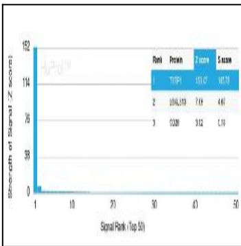
Fig. 3: Analysis of Protein Array containing more than 19,000 full-length human proteins using TYRP1-Monospecific Mouse Monoclonal Antibody (TYRP1/3282) Z- and S- Score: The Z-score represents the strength of a signal that a monoclonal antibody (Monoclonal Antibody) (in combination with a fluorescently-tagged anti-IgG secondary antibody) produces when binding to a particular protein on the HuProt™ array. Z-scores are described in units of standard deviations (SD's) above the mean value of all signals generated on that array. If targets on HuProt™ are arranged in descending order of the Z-score, the S-score is the difference (also in units of SD's) between the Z-score. S-score therefore represents the relative target specificity of a Monoclonal Antibody to its intended target. A Monoclonal Antibody is considered to be specific to its intended target, if the Monoclonal Antibody has an S-score of at least 2.5. For example, if a Monoclonal Antibody binds to protein X with a Z-score of 43 and to protein Y with a Z-score of 14, then the S-score for the binding of that Monoclonal Antibody to protein X is equal to 29.
