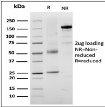
Fig. 2: SDS-PAGE Analysis Purified TYRP1-Monospecific Mouse Monoclonal Antibody (TYRP1/3282). Confirmation of Purity and Integrity of Antibody.
