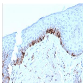
Fig. 1: Formalin-fixed, paraffin-embedded human Skin stained with TYRP1-Monospecific Mouse Monoclonal Antibody (TYRP1/3282).
