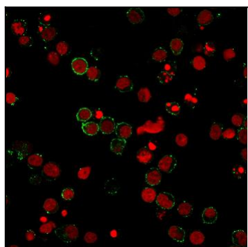
Fig. 3: Immunofluorescent staining of PFA-fixed Jurkat cells using CD31 Mouse Monoclonal Antibody (158-2B3) followed by goat anti-Mouse IgG conjugated with CF488 (green). Nuclei are labeled with RedDot (red).
