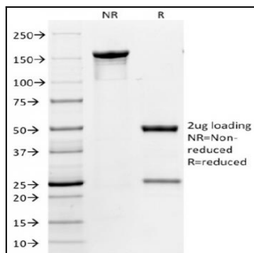
Fig. 2: SDS-PAGE Analysis Purified CD31 Mouse Monoclonal Antibody (158-2B3). Confirmation of Integrity and Purity of Antibody.
