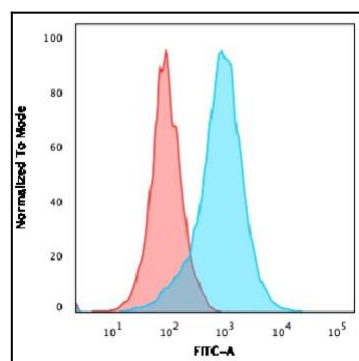
Fig. 1: Flow Cytometric Analysis of paraformaldehyde-fixed Jurkat cells using CD31 Mouse Monoclonal Antibody (158-2B3) followed by goat anti- Mouse- IgG-CF488 (Blue); Isotype Control (Red).
