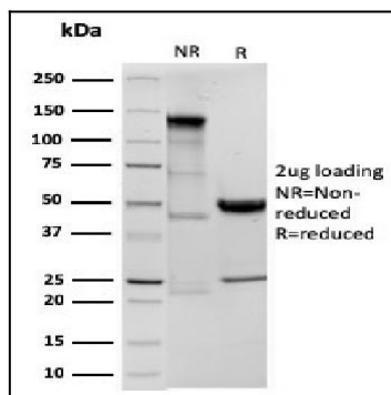
Fig. 1: SDS-PAGE Analysis Purified ODC-1 Recombinant Rabbit Monoclonal Antibody (ODC1/3636R). Confirmation of Purity and Integrity of Antibody.
