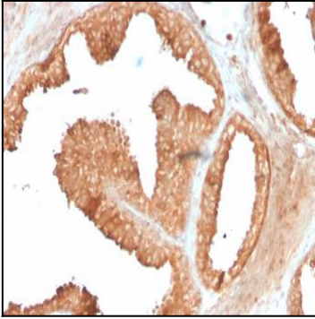
Fig. 2: Formalin-fixed, paraffin-embedded human prostate carcinoma stained with ODC-1 Recombinant Rabbit Monoclonal Antibody (ODC1/3636R).
